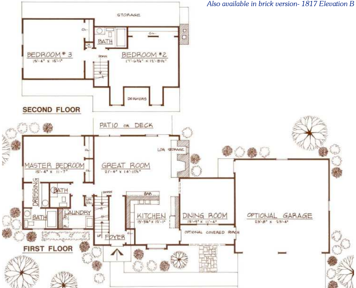
Plan 1816 (Frame) Elevation B Also available in brick version- 1817 Elevation B
